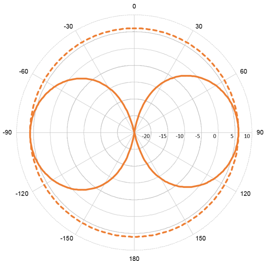
Radiation Pattern
